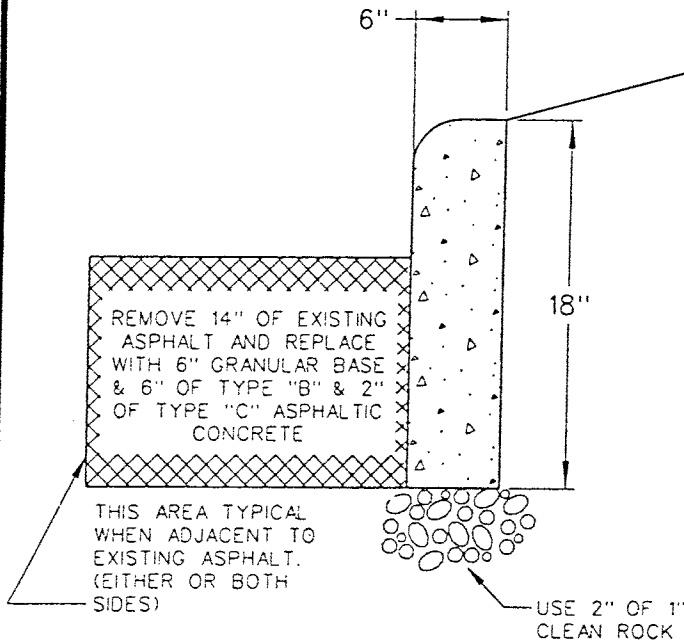
VERTICAL CURB
