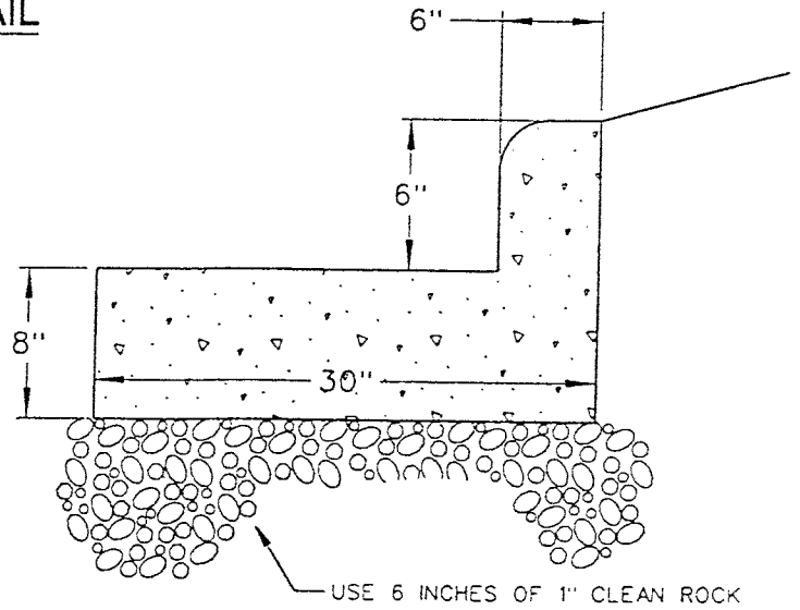
CONCRETE CURB AND GUTTER
