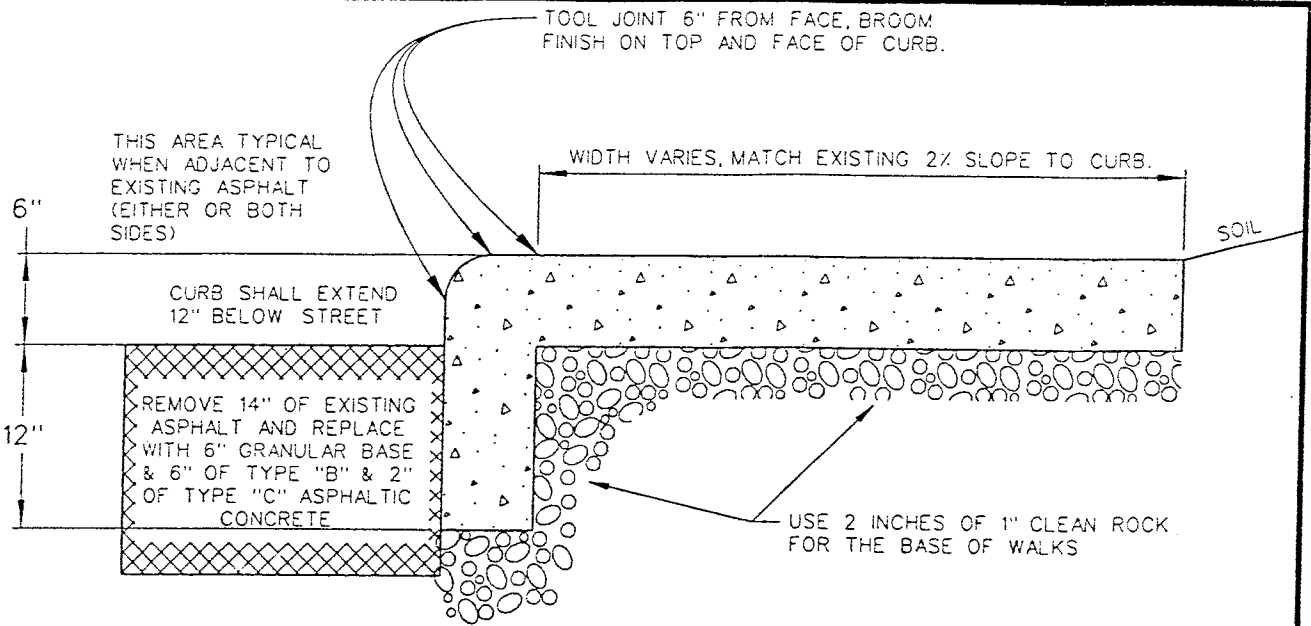
INTEGRAL CURB AND SIDEWALK DETAIL
